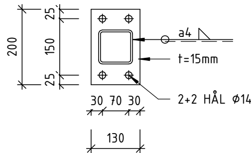
FP02 - PLAN 1 : 10
