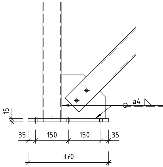
FP01 - ELEVATION 1 : 10
