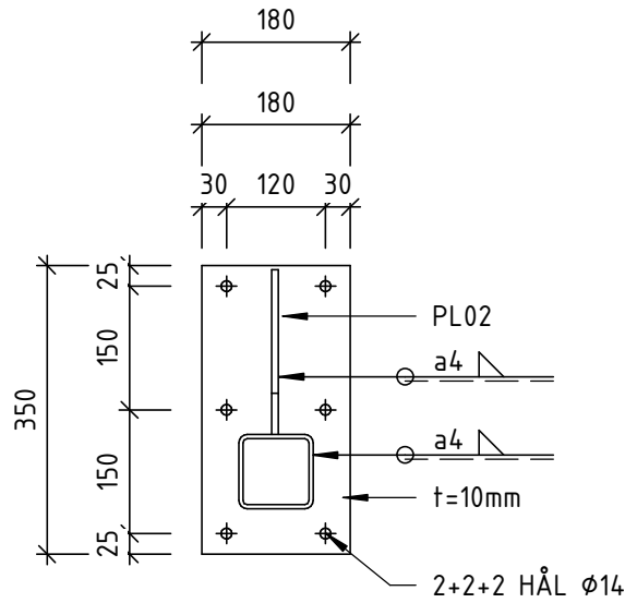
TP02 - PLAN 1 : 10
