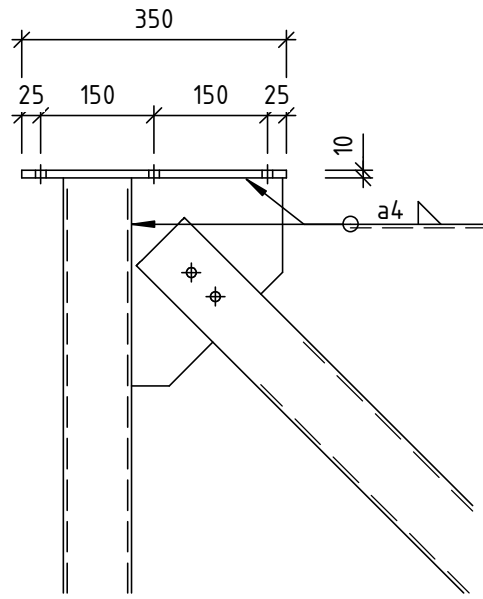
TP02 - ELEVATION 1 : 10
