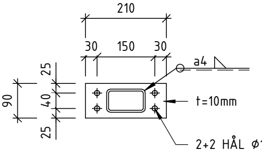
TP03 - PLAN 1 : 10
