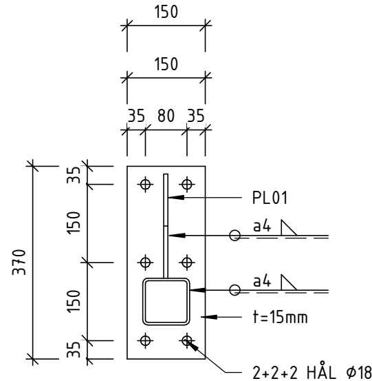
FP01 - PLAN 1 : 10
